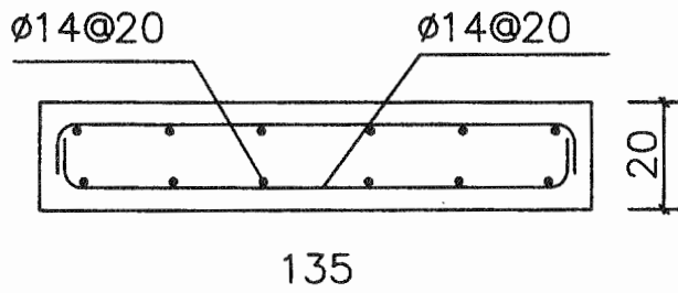
SEC.A'-A'
