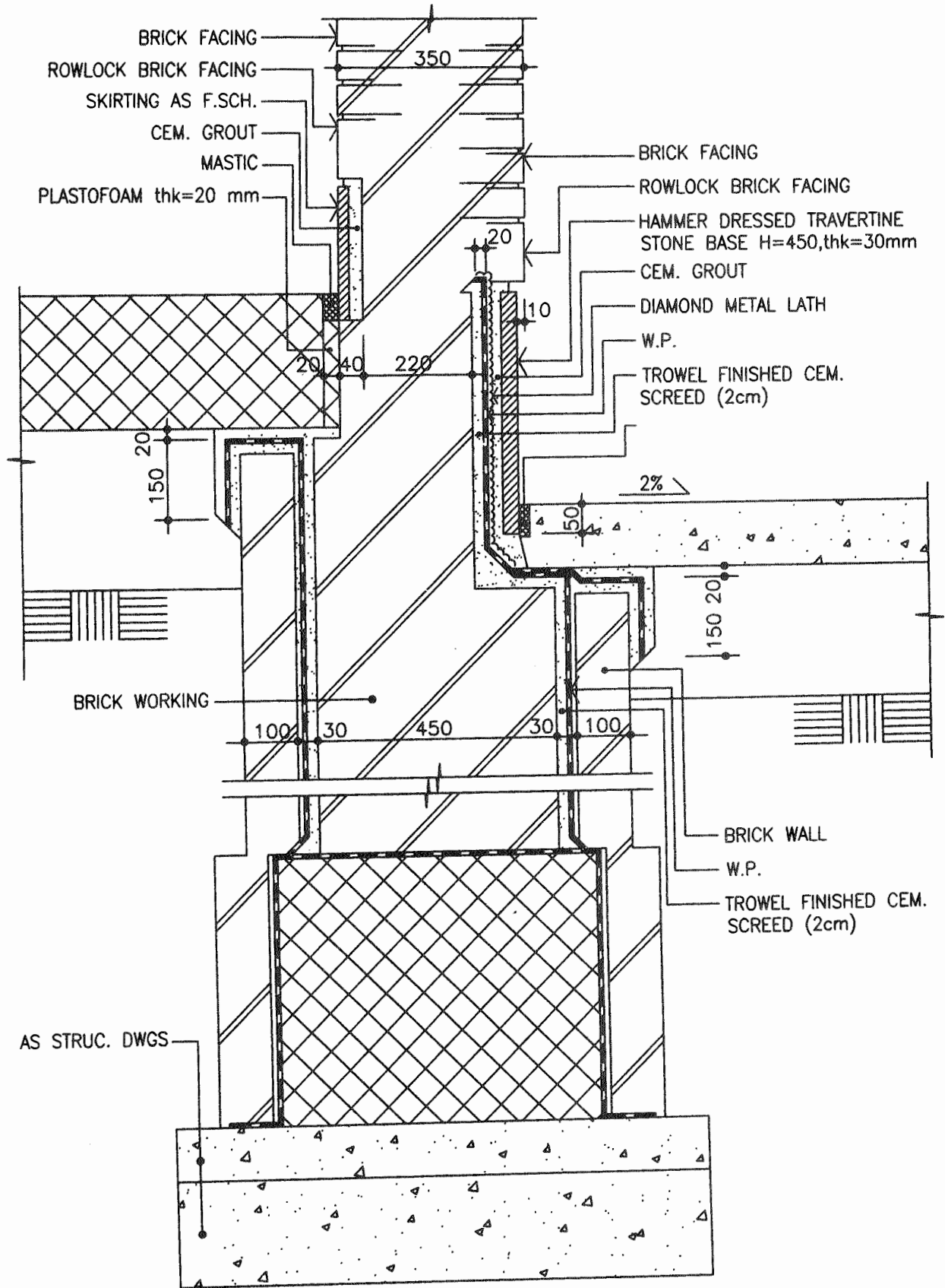
WALL SECTION
