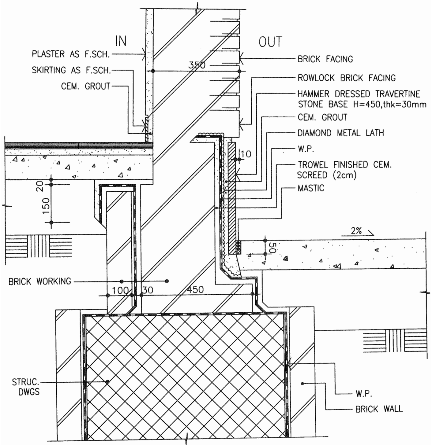
WALL SECTION
