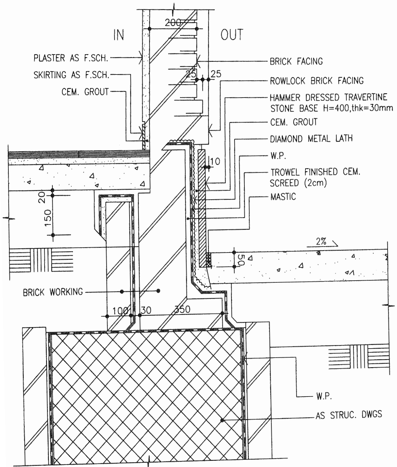
WALL SECTION
