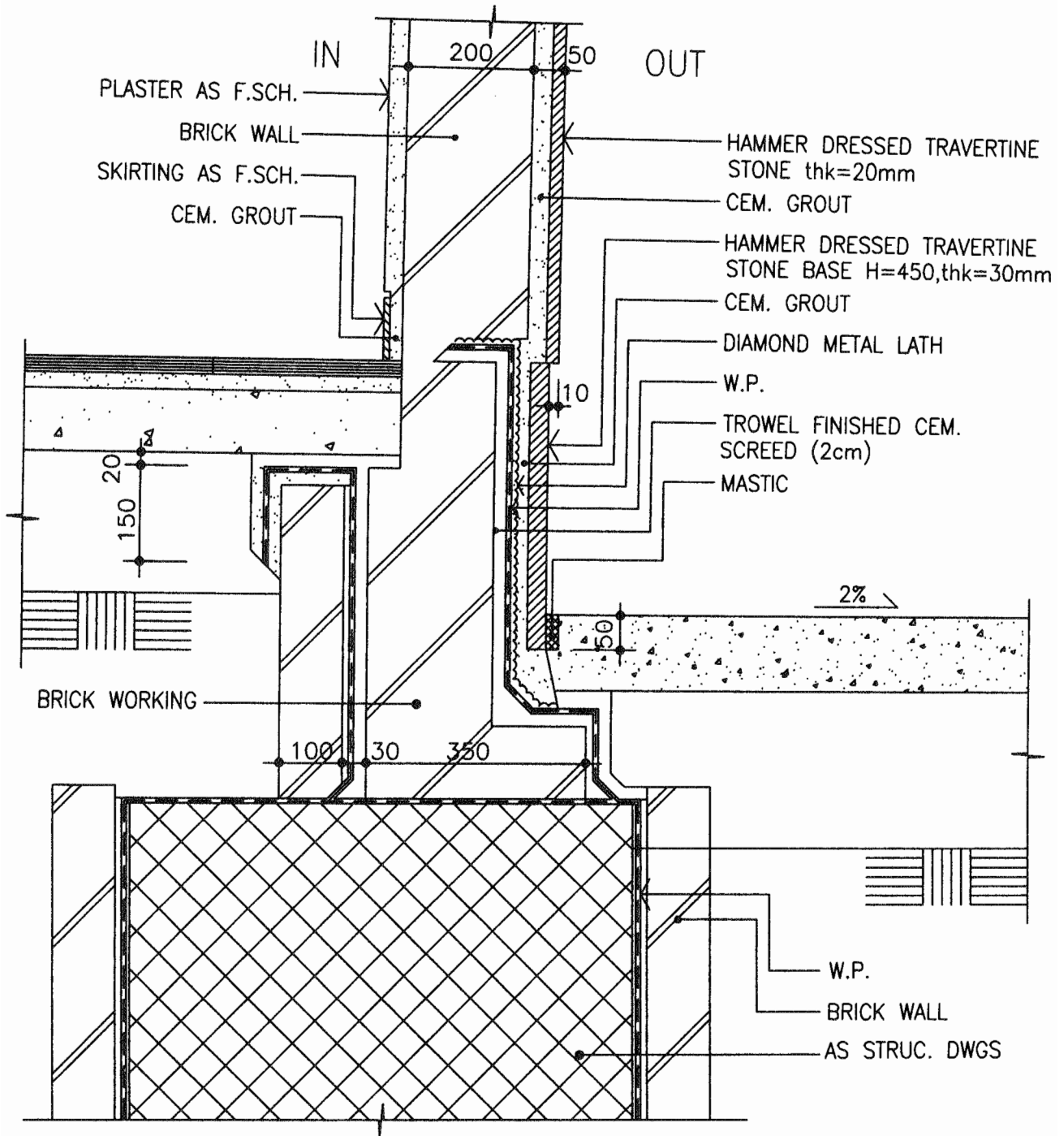
WALL SECTION
