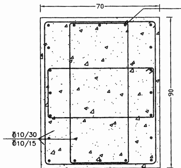
SEC. P:P
