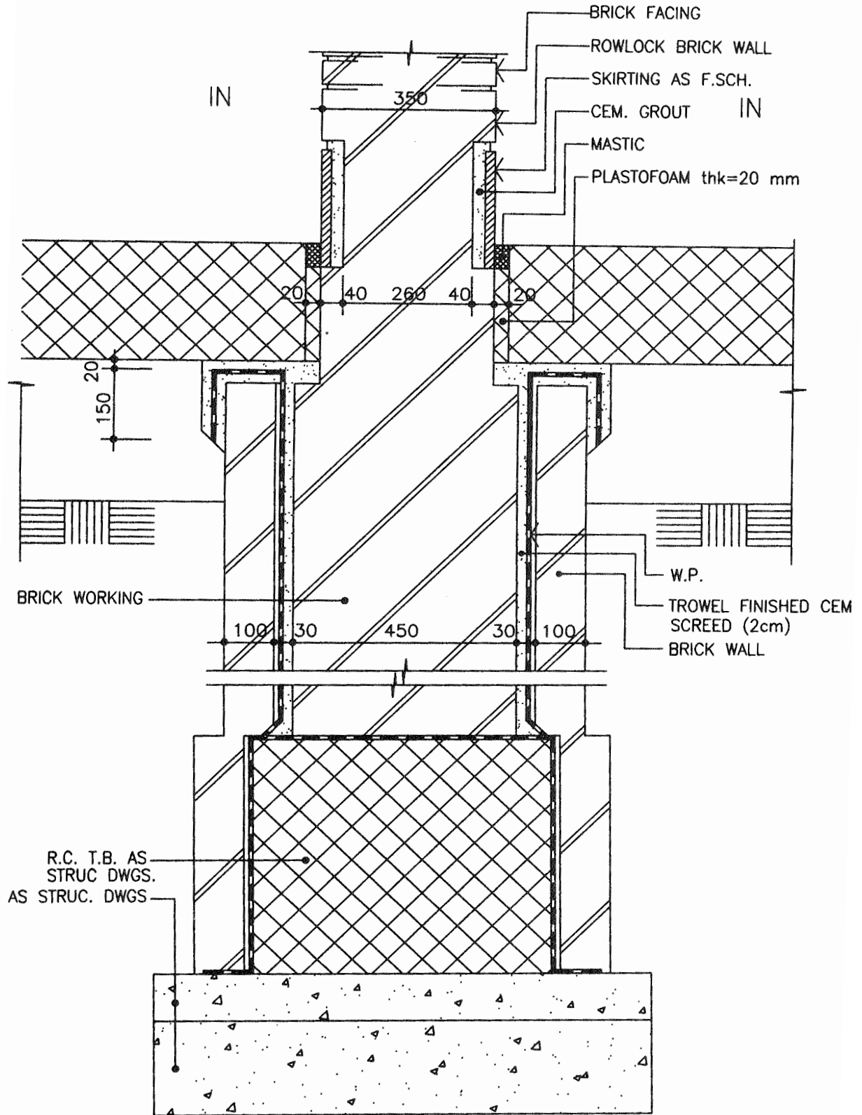
WALL SECTION
