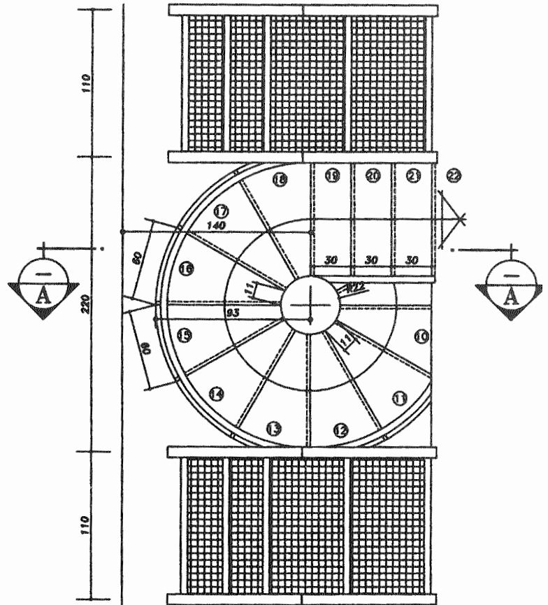
SPIRAL STAIR PLAN
