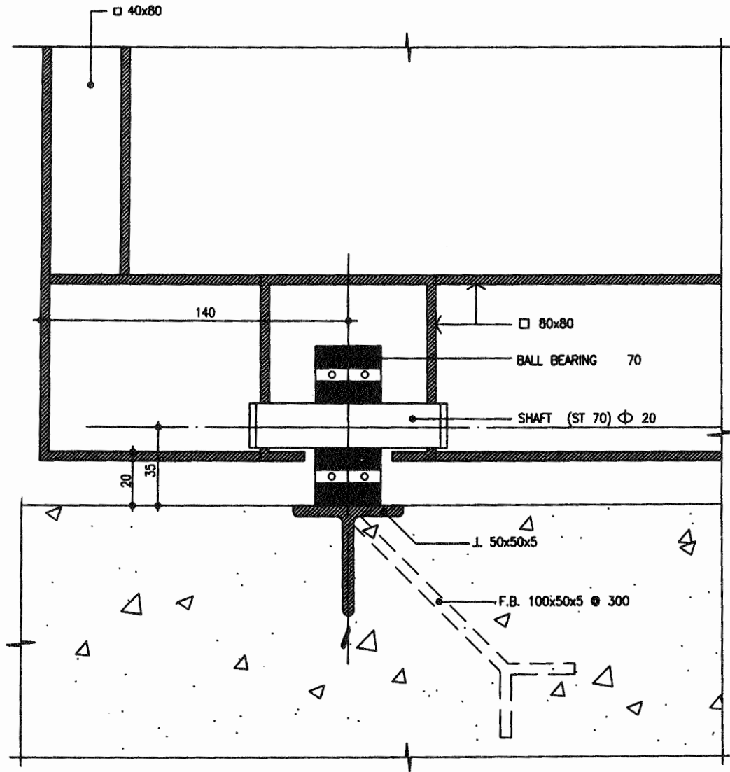
METAL DOOR WHEEL DETAIL
