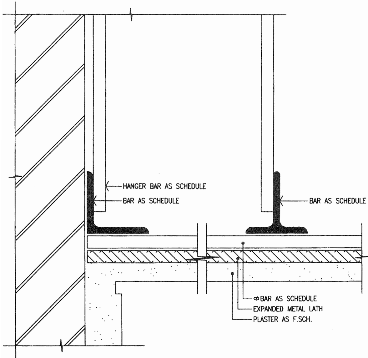
SUSPENDED CEILING
