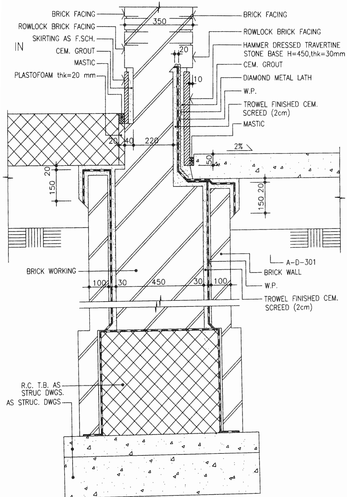
WALL SECTION
